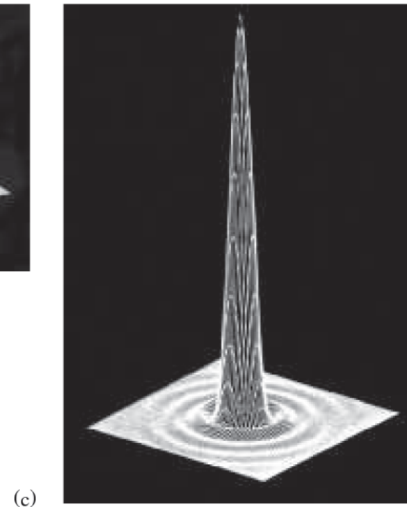
Figure 10.36 (a) The Airy pattern. (b) Electric field created by Fraunhofer diffraction at a circular aperture. (c) Irradiance resulting from Fraunhofer diffraction at a circular aperture. (R.G. Wilson, Illinois Wesleyan University)
